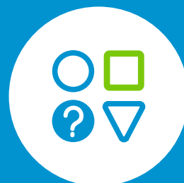
Query Categories
